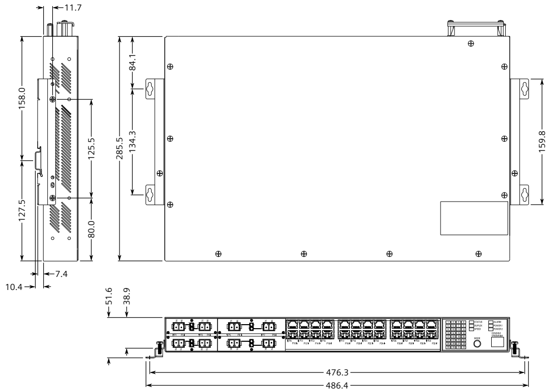
Figure 5.3 Panel and DIN Rail Mount Dimensions
